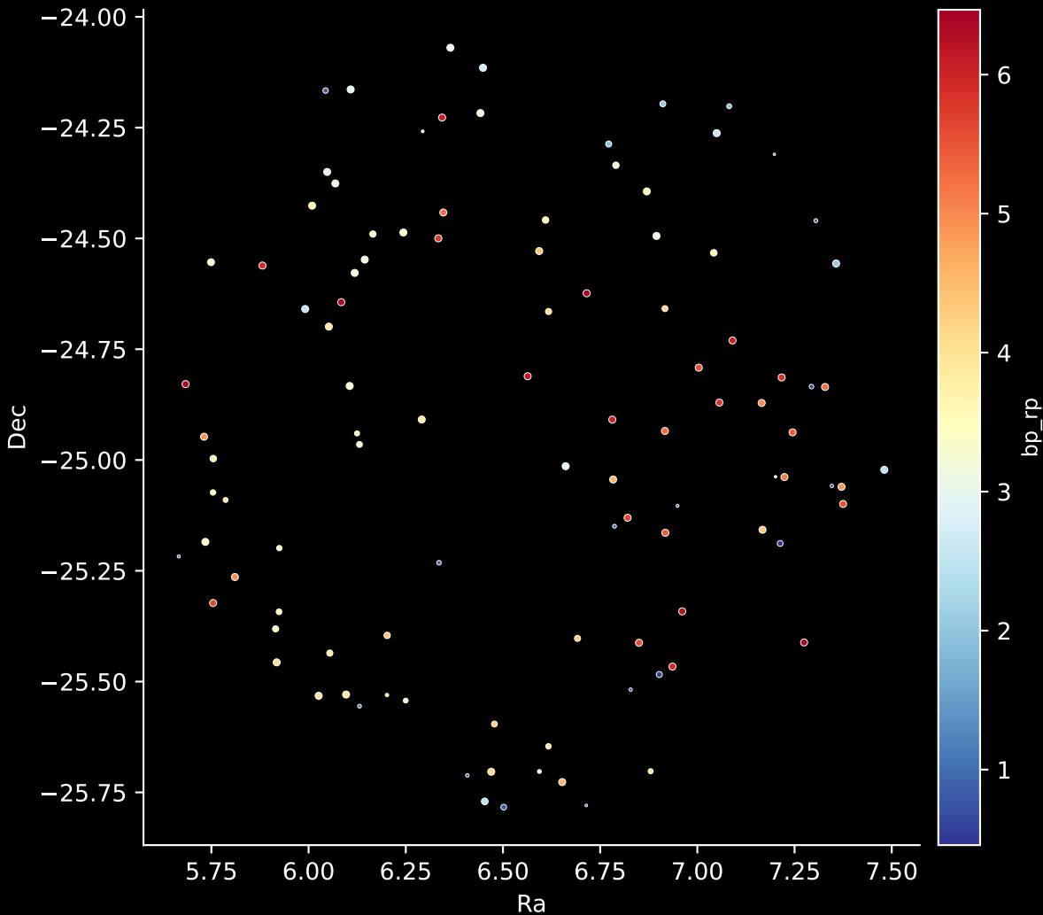
APOGEE DR17 Field: [004+02] Stars: 104
