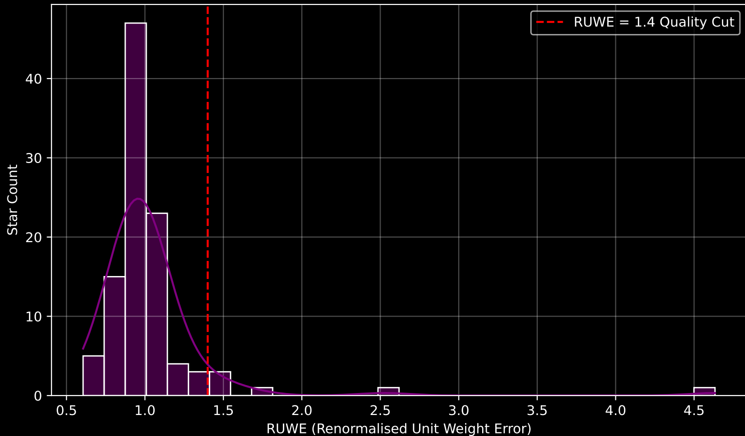
GAPOGEE DR17 Field [004+02] RUWE Distribution (n= 103)
