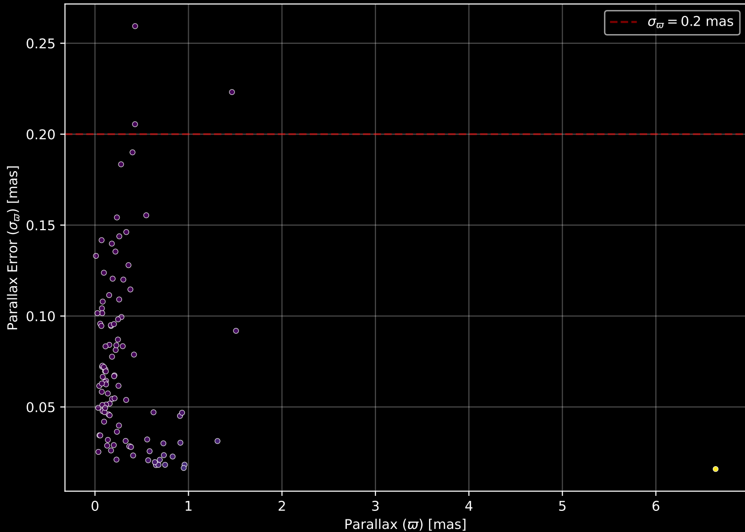
APOGEE DR17 Field: [004+02] Parallax Quality (n= 104)
