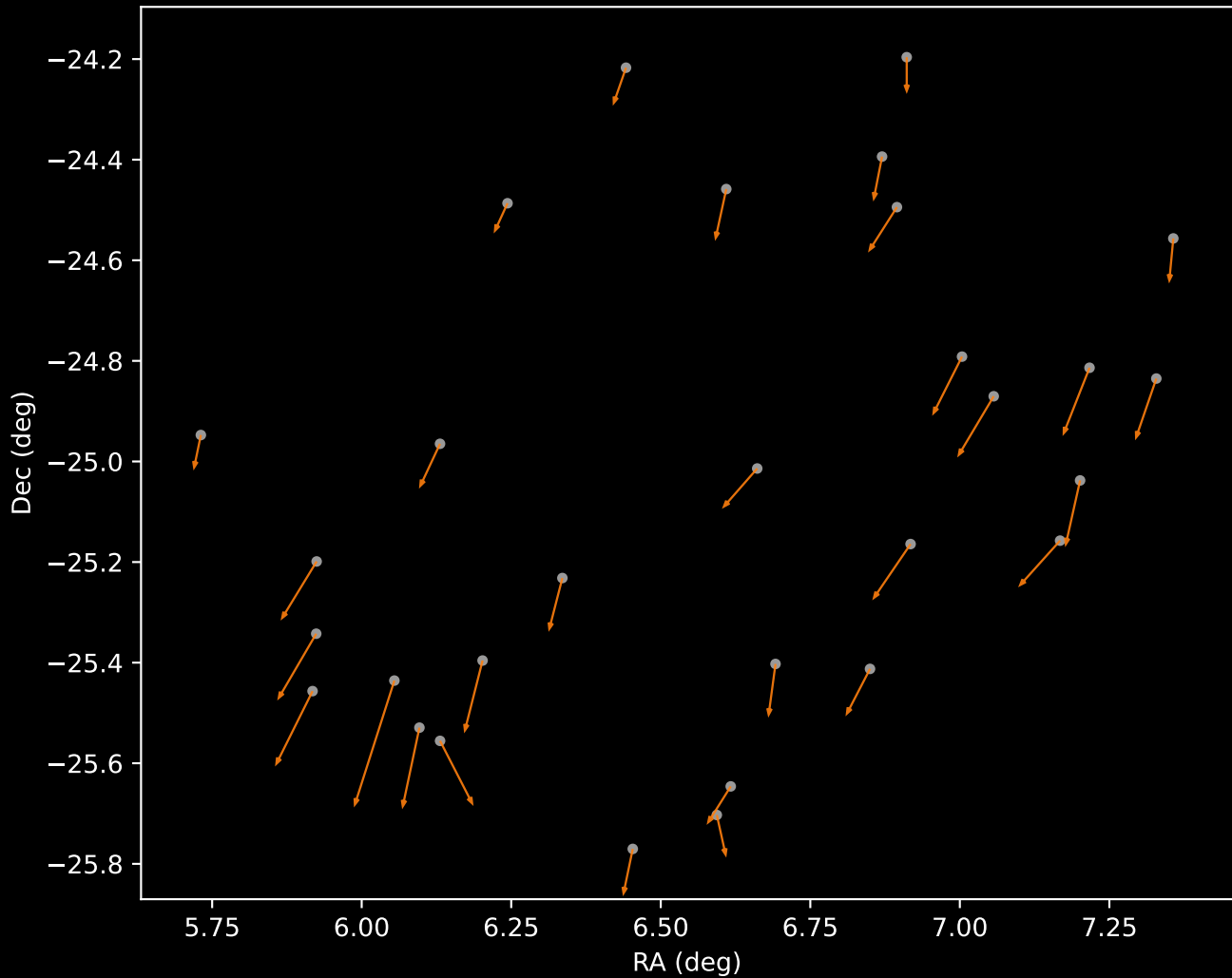
APOGEE DR17 Cluster 2 Proper Motion Vectors (n=30)
