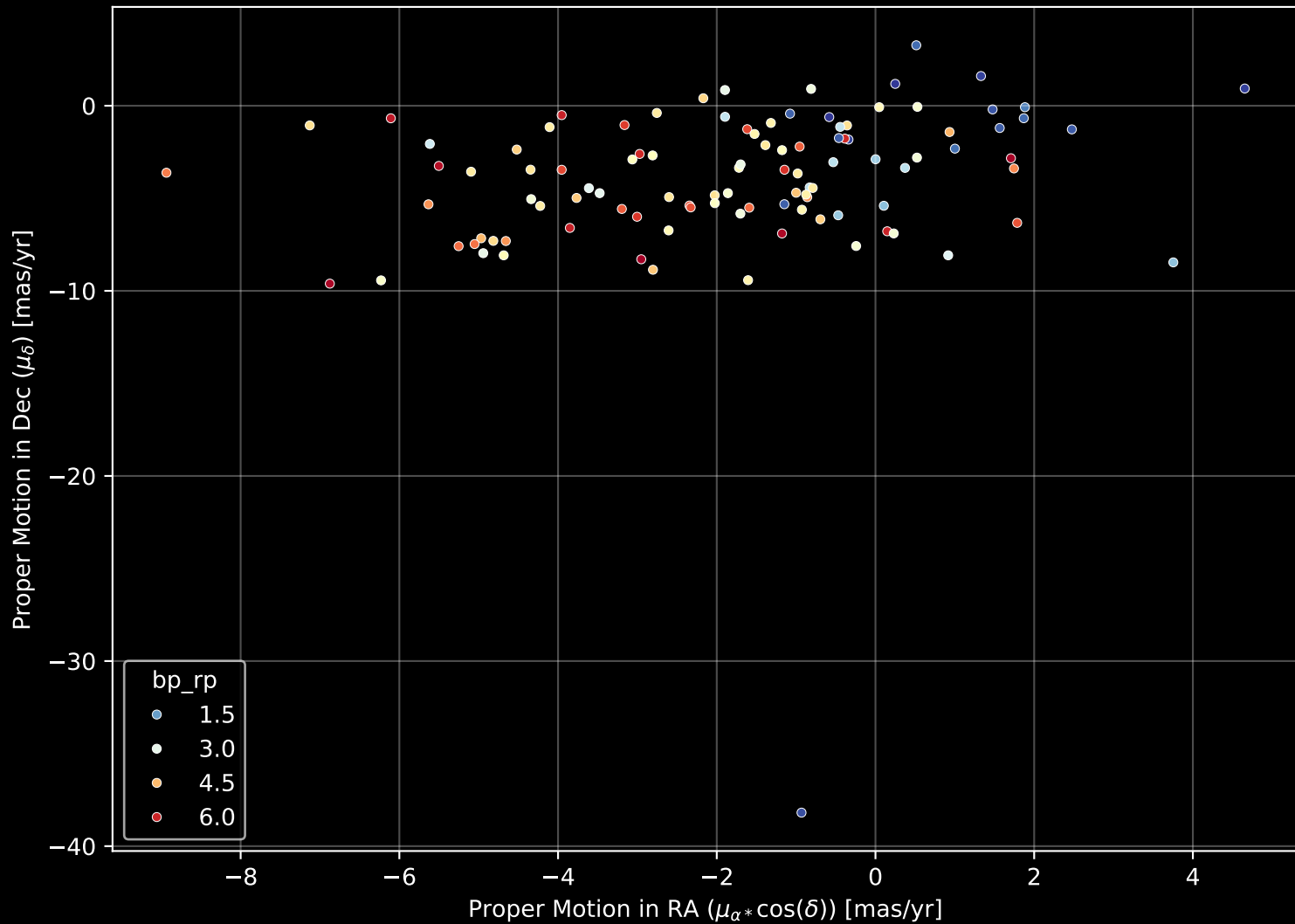
APOGEE DR17 Field: [004+02] Proper Motion Diagram (n= 104)
