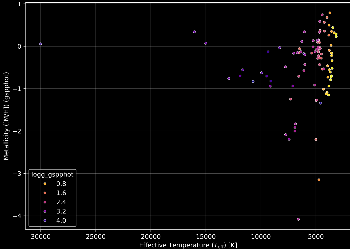
APOGEE DR17 Field: [004+02] Stellar Population Parameters (n= 104)
